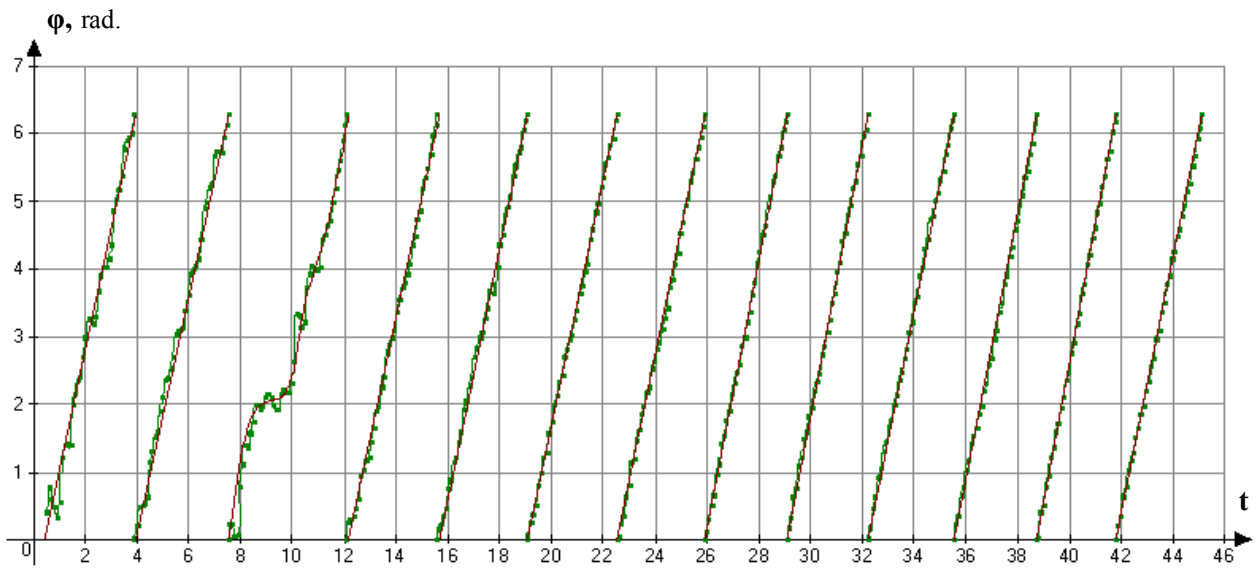
Graph 2 Dependence of polar angle \varphi on time
