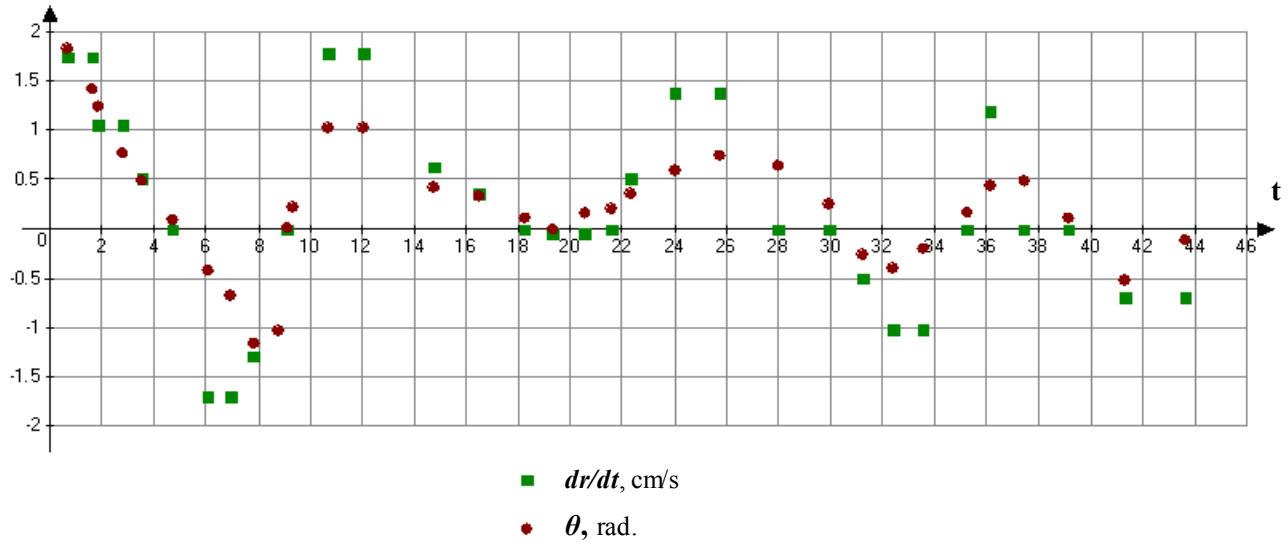
Graph 4 Dependence of rate of change of polar radius, and the angle between spin axis and the normal line to the trajectory on time
