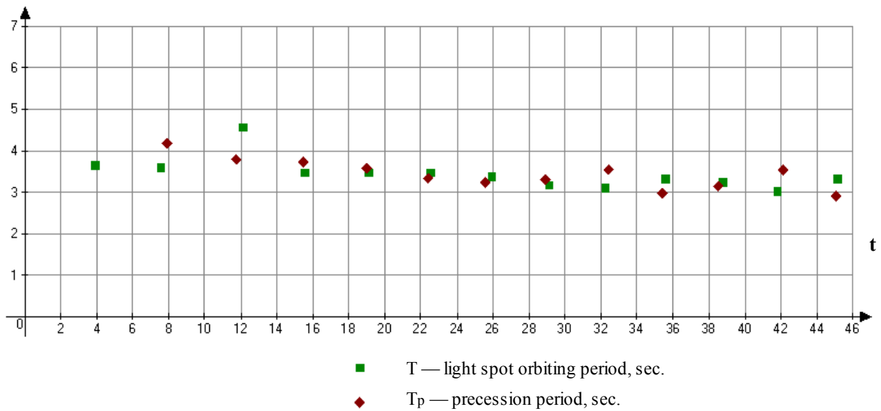
Graph 5 Dependence of the light spot orbiting period and the gyroscope precession period on time
