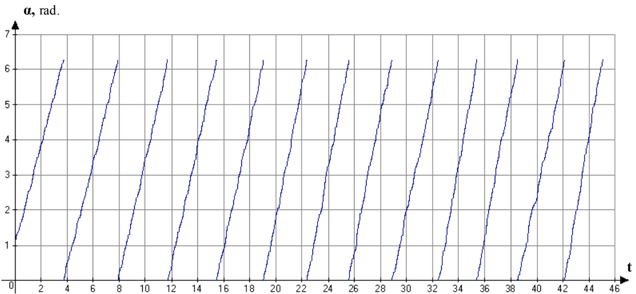
Graph 3 Dependence of the angle \alpha between spin axis of the gyroscope and the polar axis
